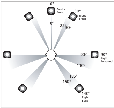
Figure 15: Recommended loudspeaker configuration for most 7.1 channel audio signals. The actual positions of the loudspeakers shows the reference placement used at Bang & Olufsen for testing and tuning.
