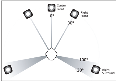
Figure 14: Standard loudspeaker configuration for 5.1 multichannel audio. The actual positions of the surround loudspeakers at 110° shows the reference placement used at Bang & Olufsen for testing and tuning. Note that the placement of the subwoofer is better determined by your listening room's acoustics, but it is advisable to begin with a location near the centre front loudspeaker.
